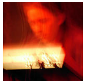
Control Theory 012
